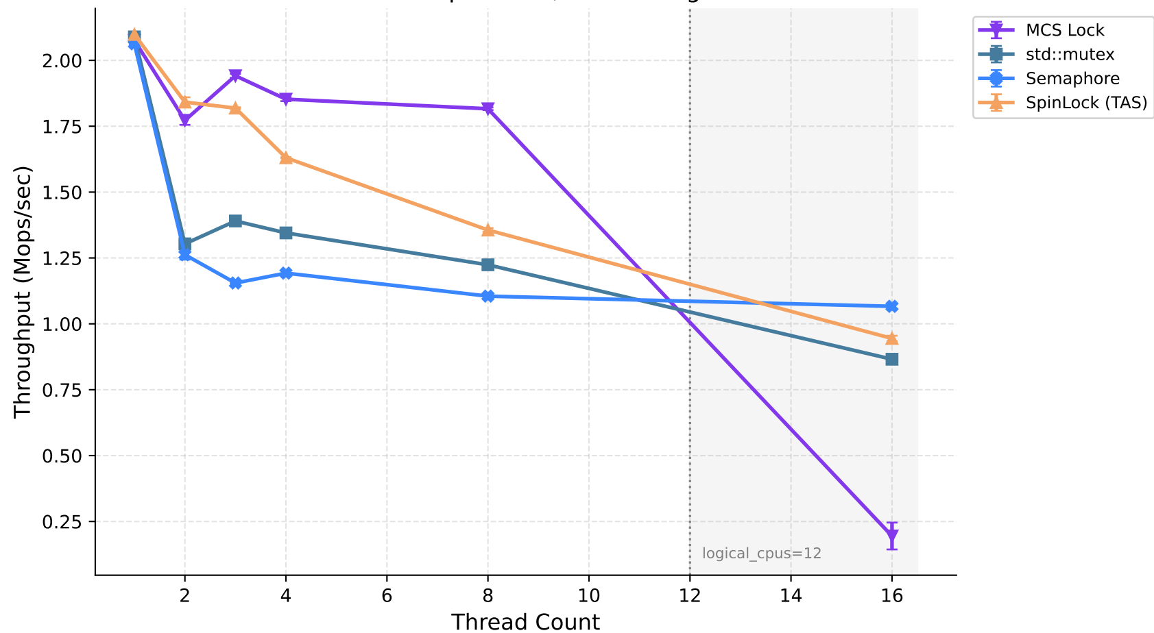
Fig 12 — Throughput Saturation Curve (CS = 500 cycles)
